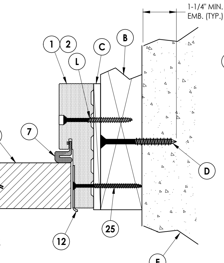
2 8 HORIZONTAL CROSS SECTION Outswing Shown (Inswing Similar) Shown w/ 2X Buck
