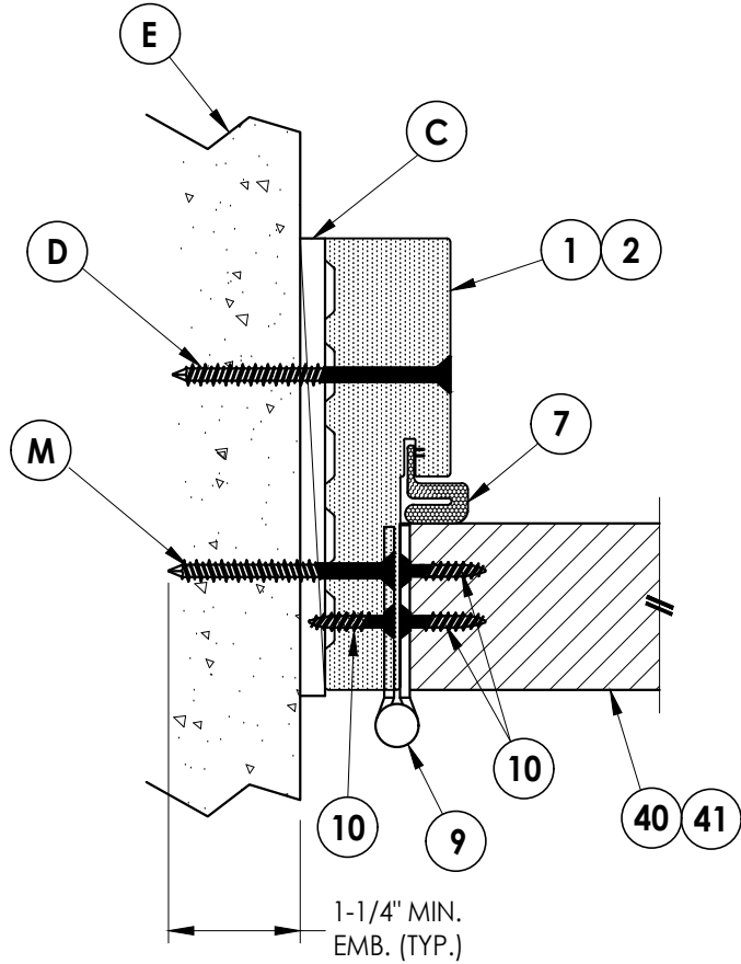
1 HORIZONTAL CROSS SECTION 10 Outswing Shown (Inswing Similar) Shown Direct to Masonry
