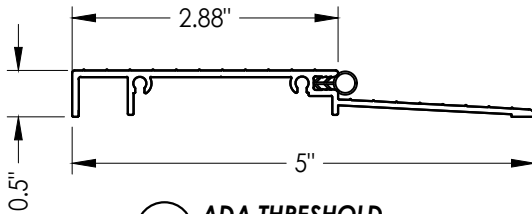
19 ADA THRESHOLD AFCO A-204T
