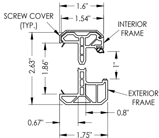
5A ODL KEYSTONE PVC LITE FRAME 1" GLAZING
