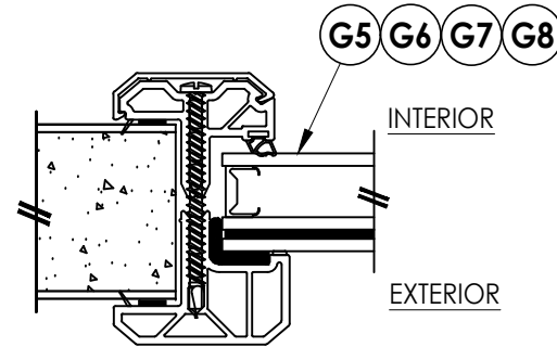
3 2 HORIZONTAL CROSS SECTION
