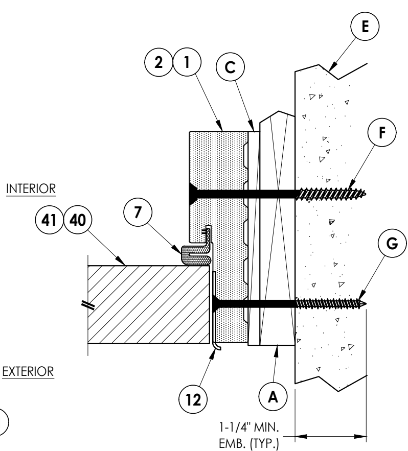
2 9 HORIZONTAL CROSS SECTION Outswing Shown (Inswing Similar) Shown w/ 1X Buck
