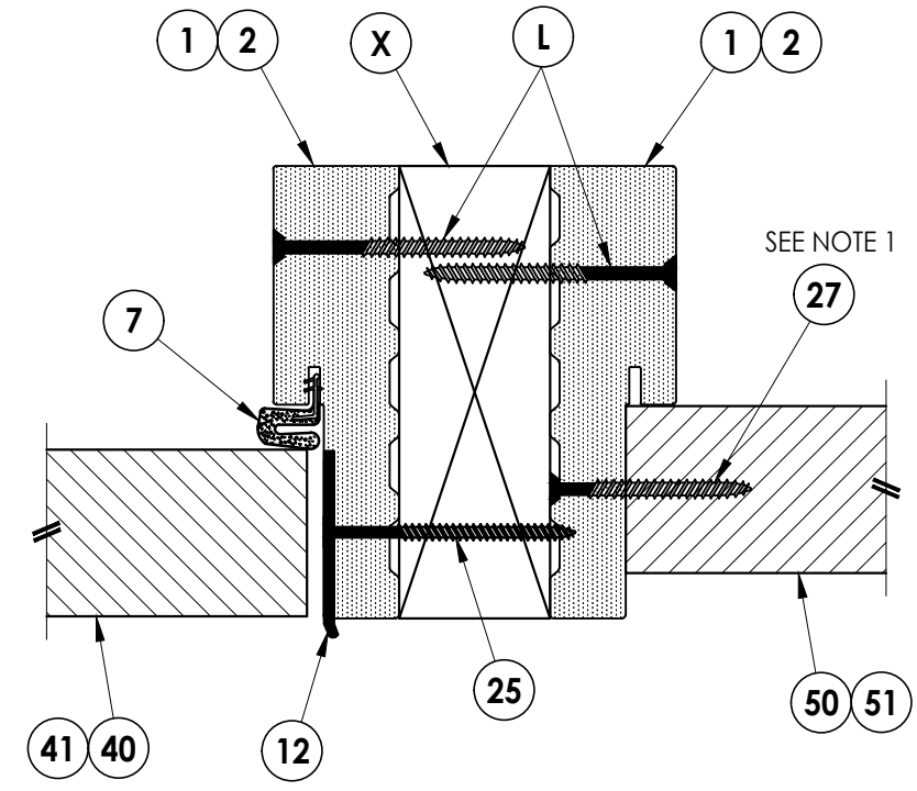
2 7 HORIZONTAL CROSS SECTION Outswing Shown (Inswing Similar)
