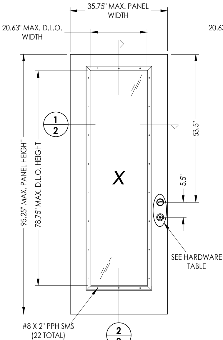
40 FIBERGLASS DOOR PANEL ODL w/ FLAT ALUM. LITE FRAME
