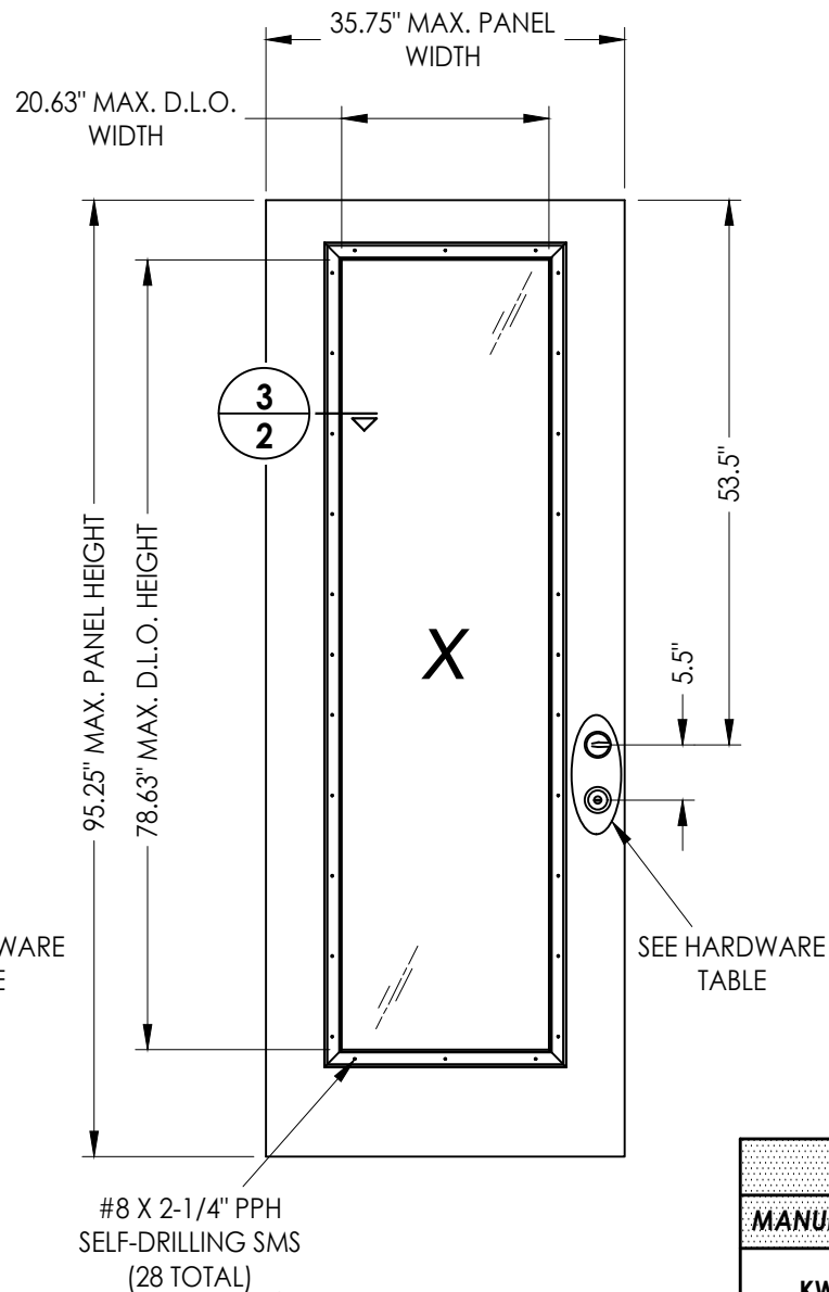
41 FIBERGLASS DOOR PANEL ODL w/ KEYSTONE PVC LITE FRAME
